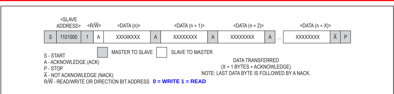
Figure 4. Data Read—Slave Transmitter Mode
